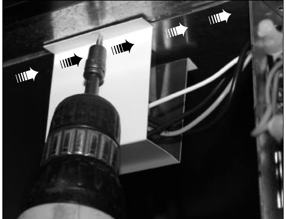
Figure 10. Anchoring Relay Shield
