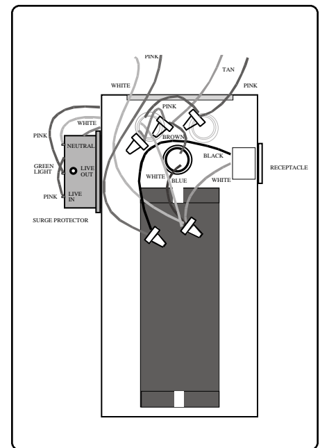
Figure 3 Ballast Box Before Surge Protector
