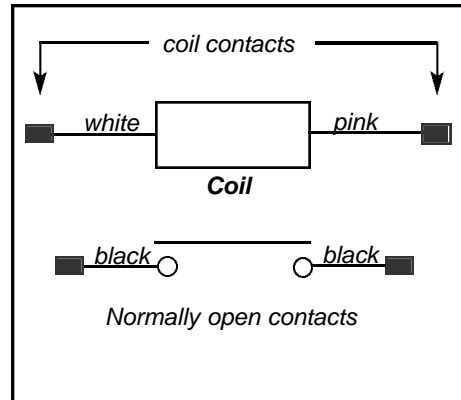
Figure 6. Relay Wiring Diagram
